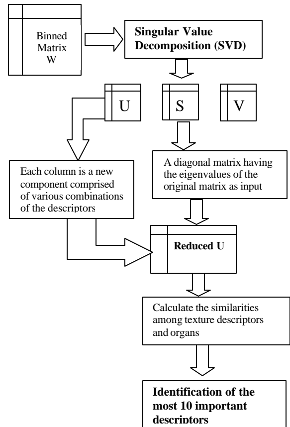
Figure 2: The feature discrimination identification process
